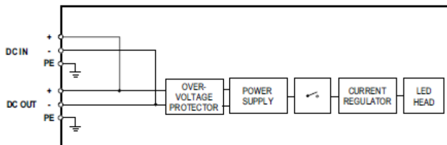
LI-170-048-F block diagram
